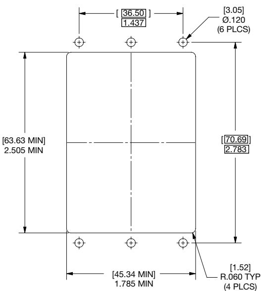
SIZE 2: RECEPTACLE
