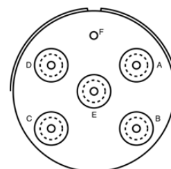
24-79 Solder Coax 5 1 8 20
