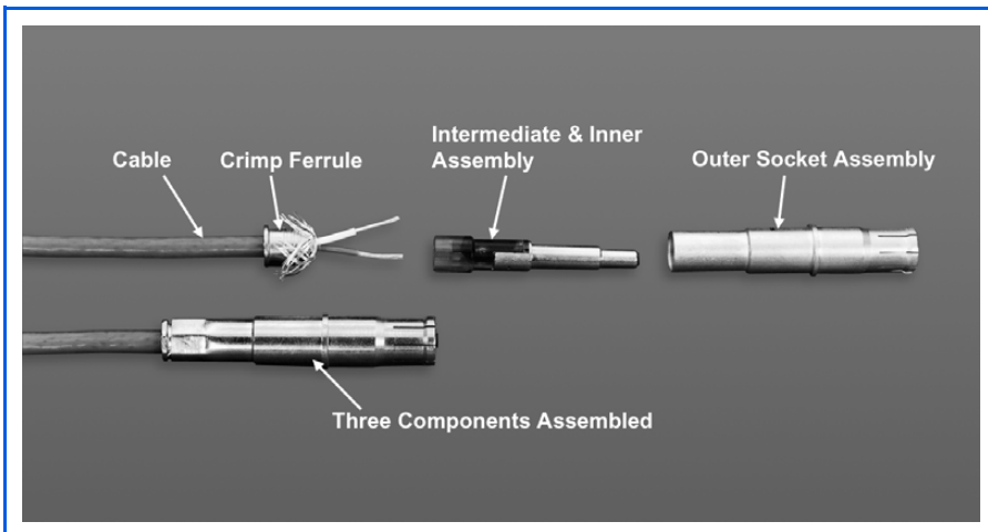
RCT (Reduced Component Twinax Size 8 Contact
