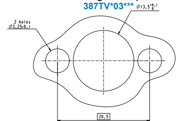
Oval flange receptacle 387TV*03***
