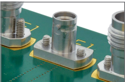
Available in threaded and push-on series (SMPM Shown)
