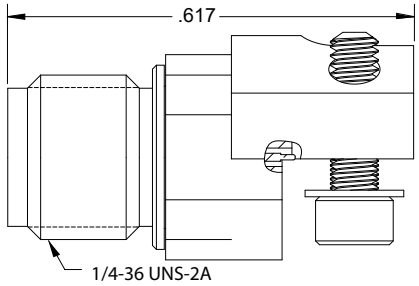
SMA Solderless Edge Launch Connector P/N: SF2921-61450
