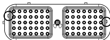
70 Pos Plug - Key C
