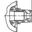
VIEW D FOR SIZE 8 TWINAX ONLY, RELATIVE TO -A- .940 MAX 23.88 MAX
