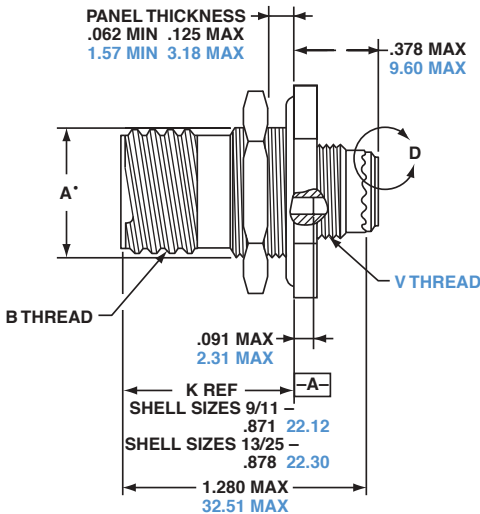
VIEW D FOR SIZE 8 COAXIAL ONLY, RELATIVE TO -A- .794 MAX 20.17 MAX
