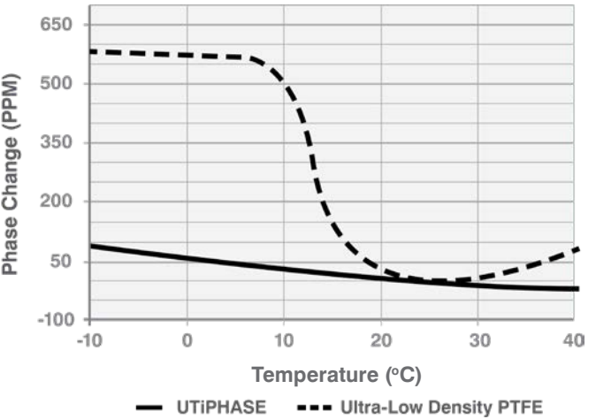
Fig 2: Typical phase change vs. temperature for flexible microwave cables
