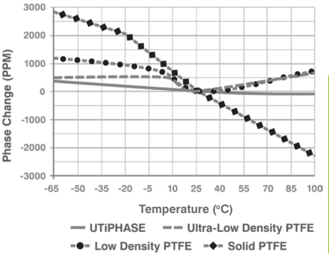
Fig 3: Typical phase change vs. temperature for flexible microwave cables with different dielectrics
