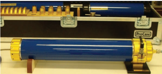
In-house RF shielding & transfer impedance testing
