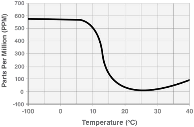
Fig 1: Typical phase change vs. temperature for cables with ultra-low-density PTFE dielectric
