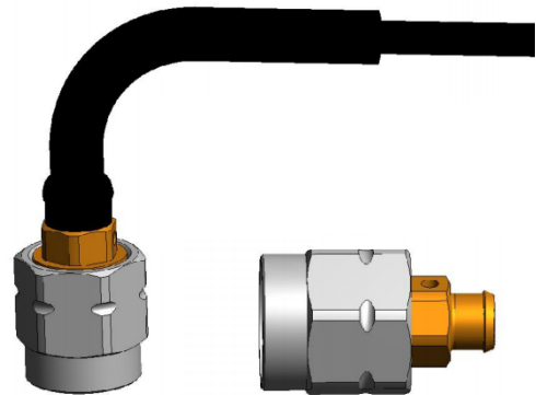
Precision-formed ends for optimal electrical performance
