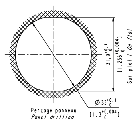
Panel drilling
