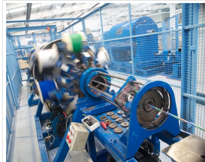
Cable lay-up machine, subsea cable manufacturing
