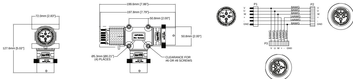
FIG 8: Tee, Angled Leg, Black
