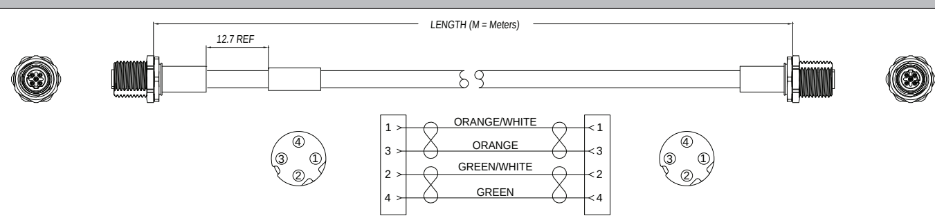
FIG 7: P29931-Mxxx, Ethernet M12, Female to Female, Receptacle, Orange
