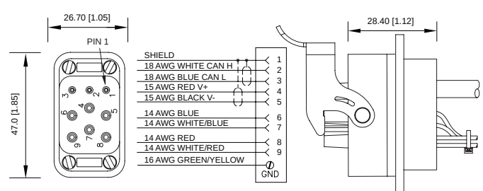
FIG 6: Female Power, Receptacle, Straight, 9 Position
