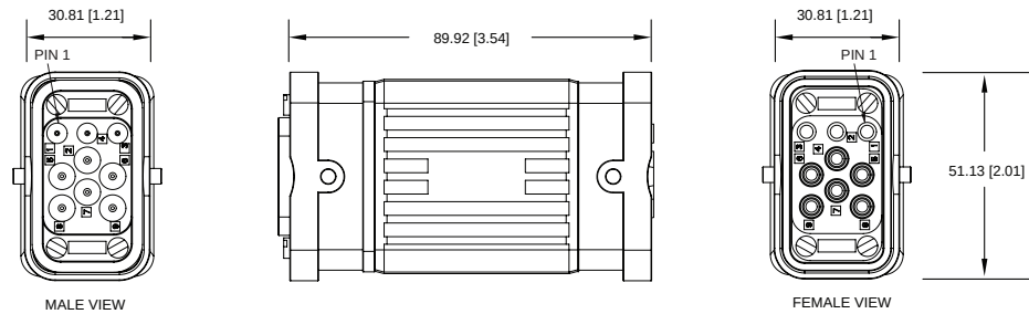
FIG 9: Male, 120V, Terminator, 9 Position
