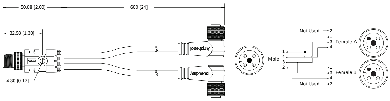
FIG 9: Male Straight to Female 90°, Splitter - (1) 4 Pos. to (2) 4 Pos.
