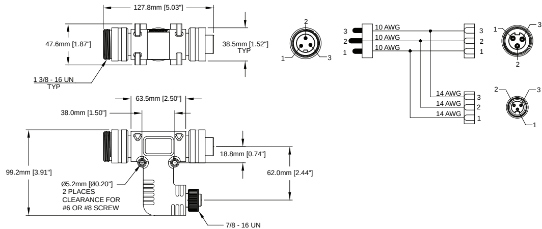
FIG 12: "h" Reducing Tee, 3 Position
