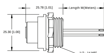
FIG 16: Female, Terminating Plug, Straight, 5 Position
