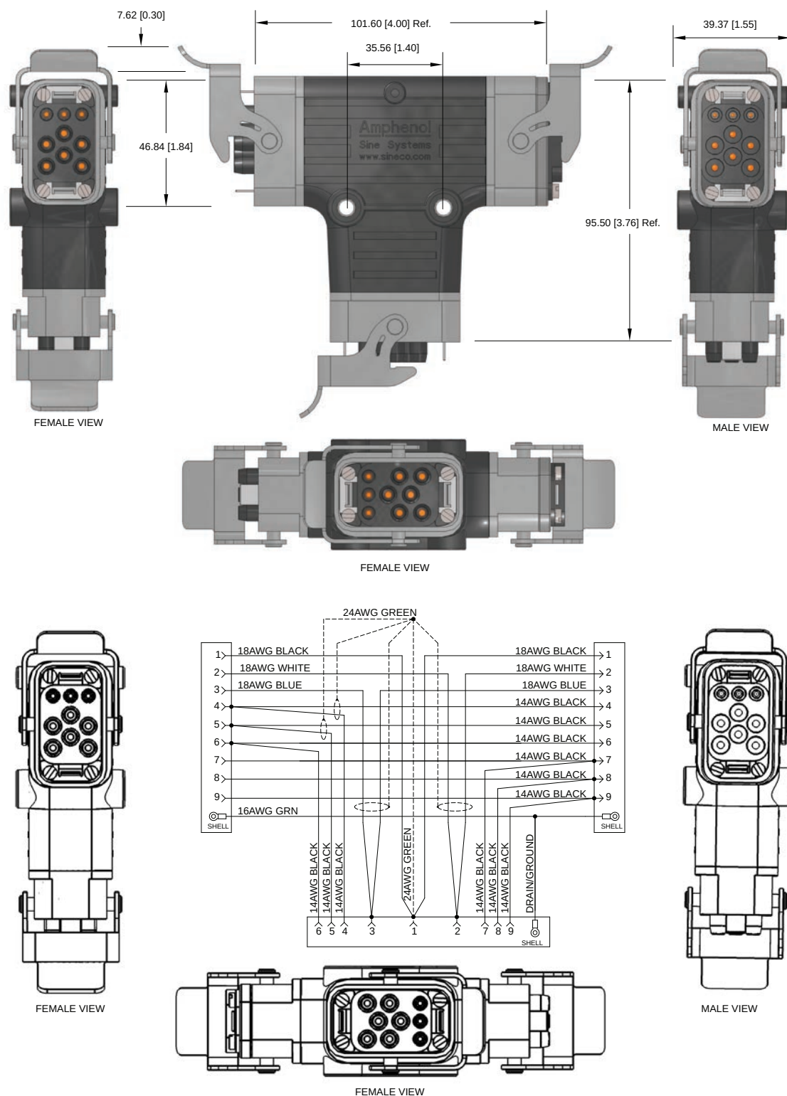
FIG 7: Hybrid Tee, 600V, 9 Position
