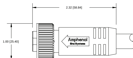
FIG 2: Female, Plug, Straight, Internal Threads
