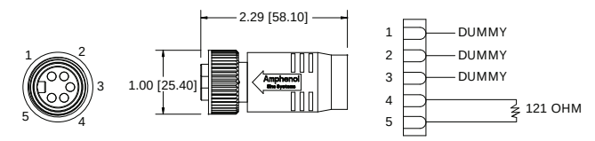
FIG 16: Female, Terminating Plug, Straight, 5 Position
