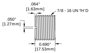
FIG 13: Threaded Union
