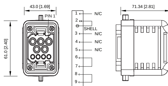
FIG 11: Male, Dual Channel, Terminator, 9 Position
