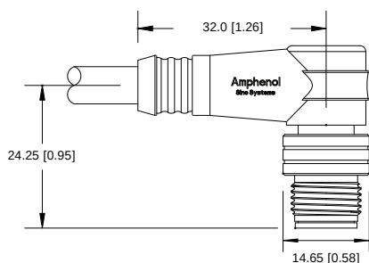
FIG 3: Male, Plug, 90°, External Threads
