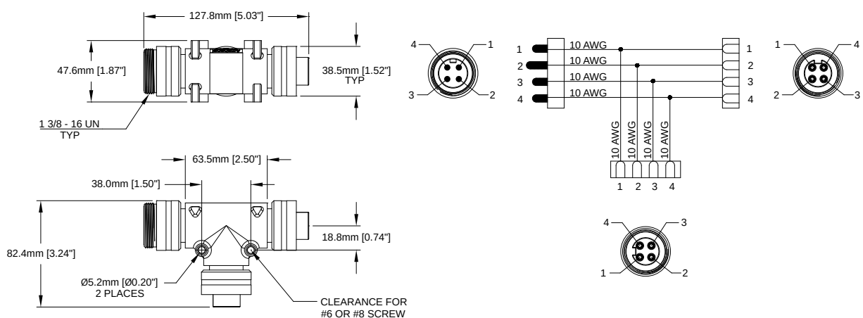
FIG 14: Tee, 4 Position
