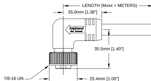
FIG 4: Female, Plug, 90°, 6P/5U
