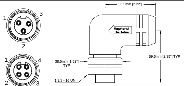
FIG 4: Female, Plug, 90°, Trunk, 3 and 4 Position
