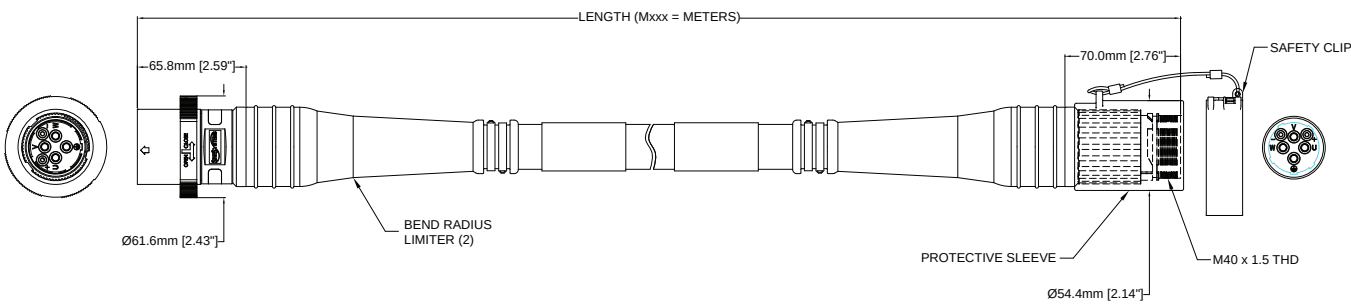
FIG 4: Male, Straight, Receptacle
