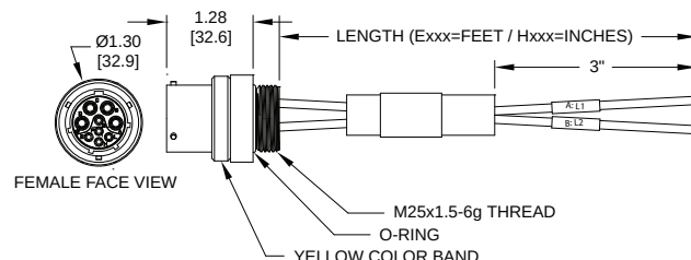
FIG 5: Female, Receptacle, Straight, 9 Position
