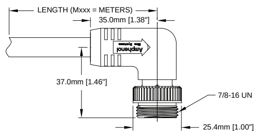
FIG 3: Male, Plug, 90°, 6P/5U
