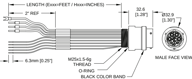
FIG 4: Male, Receptacle, Straight, 9 Position
