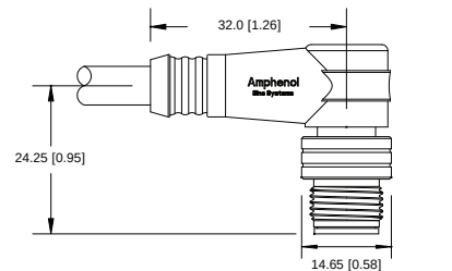
FIG 9: Male, Mini, Receptacle, Thick, External Threads
