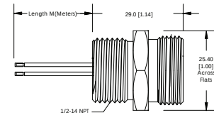
FIG 12: Female, Mini, Receptacle, Thick, Internal Threads
