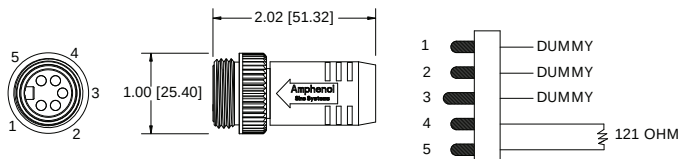
FIG 15: Male, Terminating Plug, Straight, 5 Position
