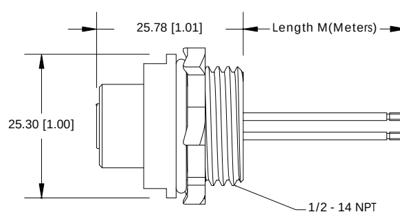
FIG 6: Female, Receptacle, Straight, Internal Threads
