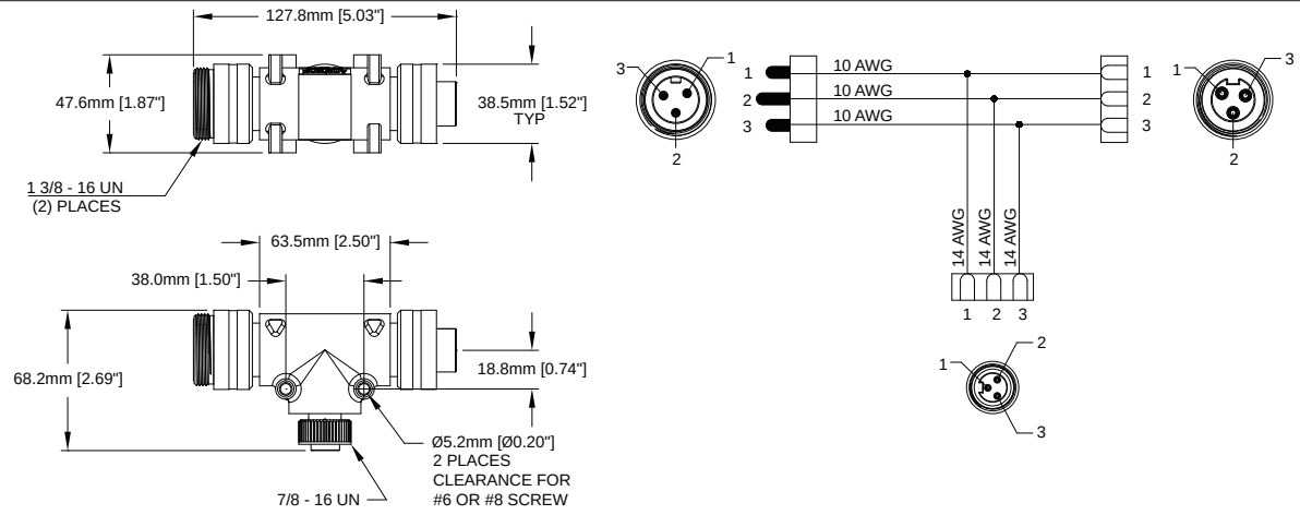
FIG 11: "h" Tee, 3 Position
