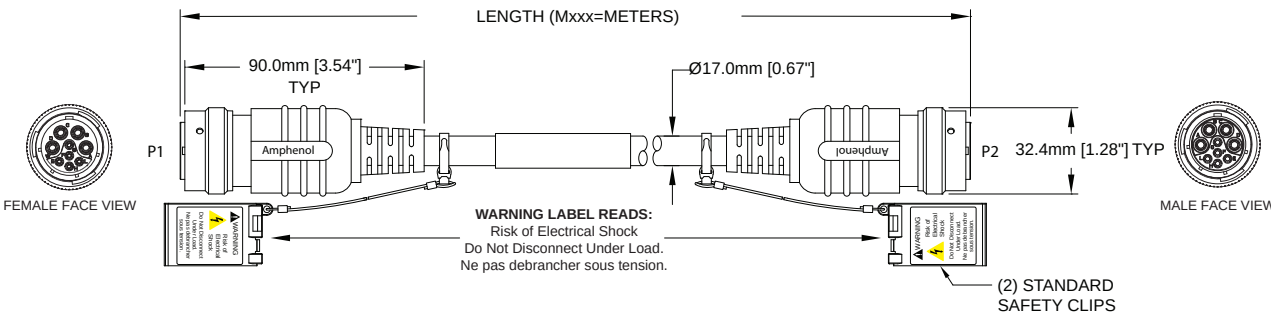
FIG 3: Male Plug to Female Plug, Straight, 9 Position
