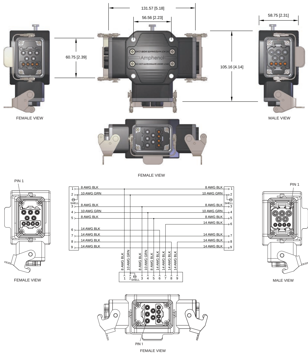
FIG 8: Dual Channel Tee, 600V, 9 Position
