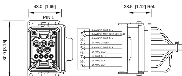
FIG 5: Male Power, Straight, Receptacle
