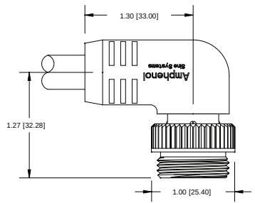
FIG 7: Female, Receptacle, Internal Threads
