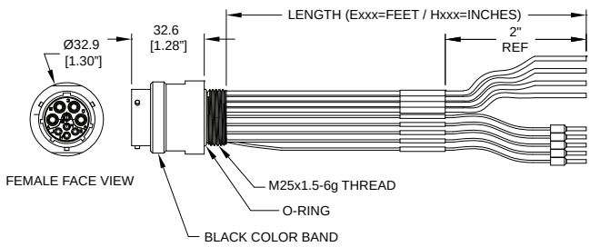
FIG 5: Female, Receptacle, Straight, 9 Position
