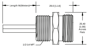
FIG 11: Male, Micro, Receptacle, Thin, External Threads
