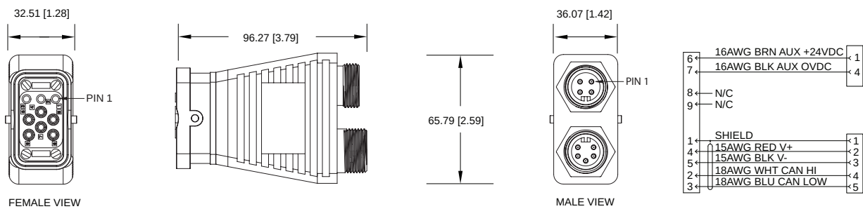
FIG 13: Female to Male, 9 Pos., 4 Pin Tap
