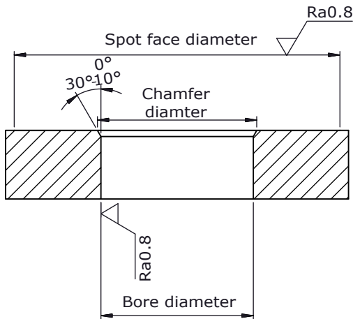
Mounting Requirements
