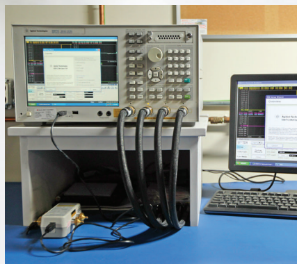
Agilent Technologies network analyzer
