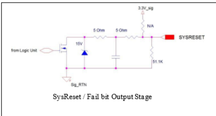
Figure 2 – SysReset and Fail Bit Output Stage
