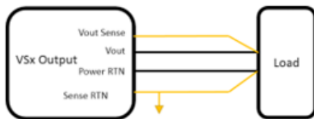
Figure 3: PSVA6USTPU115P1100-0 Sense Lines
