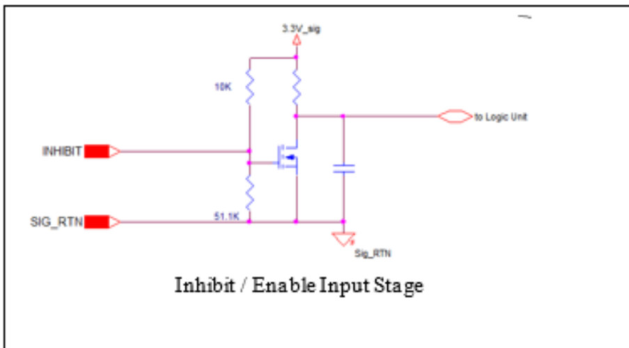
Figure 1 – Inhibit and Enable Input stage
