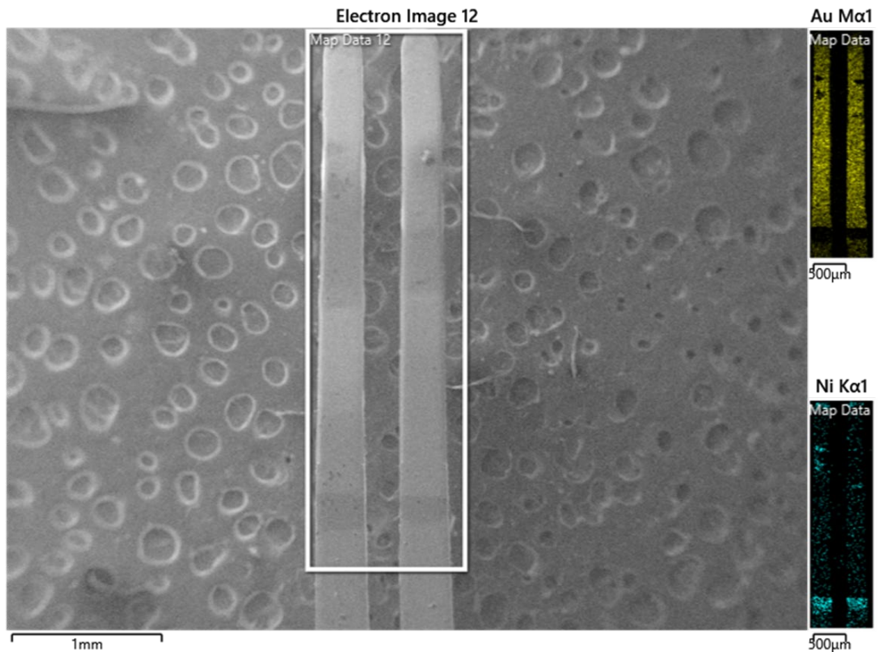
Figure 3.5-4: SEM w/EDS map Contact J8 Row E
