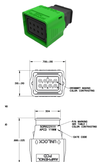
Plug Shell size 2
