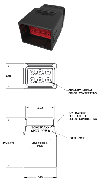
Receptacle Shell size 2
