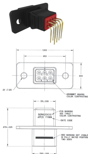
Front Flange Mount Shell size 2
