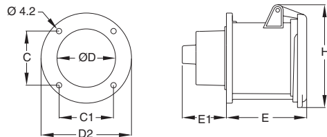
Dimensions (mm)
