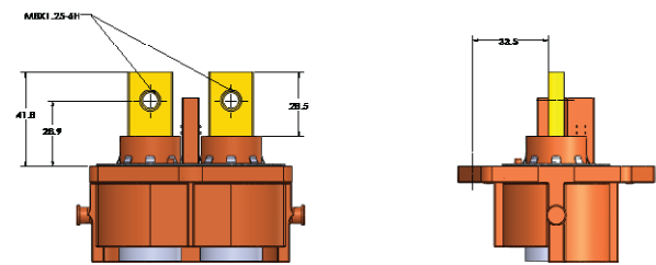
Busbar Type 1
