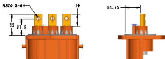
Busbar Type 1
