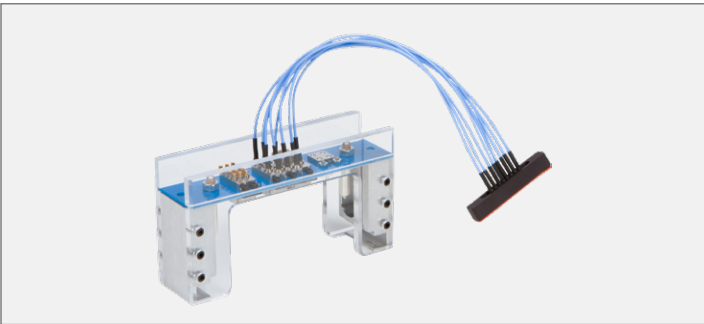
Figure 5 VITA Sample Chassis with SMPM Backplane Connector Modules terminated to Mini-D RF Bulkhead Mount IP68 8-Port SMPS Male Connector with Ø.047” Flex Cable
