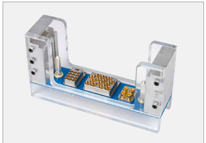
Figure 1 VITA Sample Chassis with 67.1/67.2 (SMPM) and 67.3 (SMPM & SMPS) Modules
