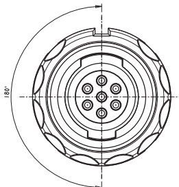
Plug keyway orientation
